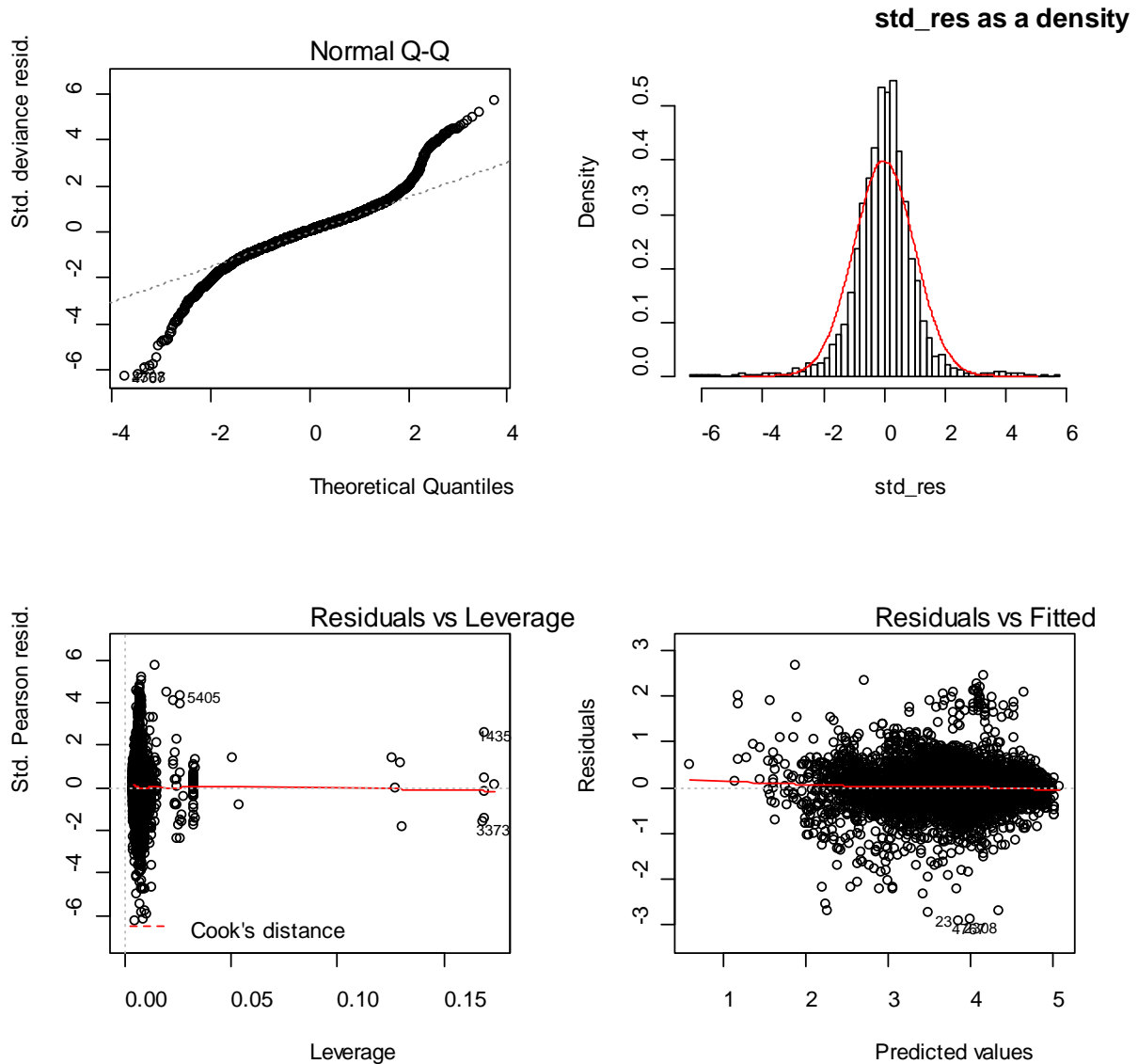
Figure B1: Diagnostic plots describing the fit of a standardised model of scallop catch rates for the Rangaunu Bay scallop fishery. A quantile-quantile plot of standardised residuals [upper left panel]; a histogram of the standardised residuals compared to the distribution predicted from a lognormal distribution [upper right panel]; a plot of standardised residuals against the leverage that each data point has on the modelled relationship between daily catches and explanatory variables [lower left panel]; standardised residuals plotted against predicted daily catches [lower right panel].
