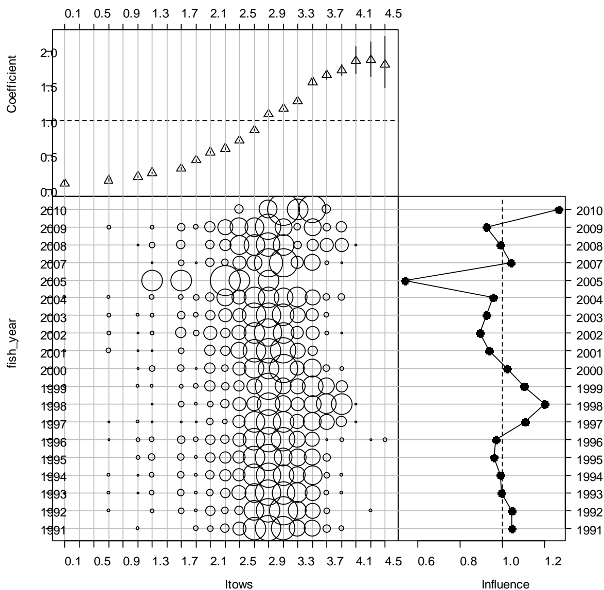
Figure B2: Effect of the logged number of tows (per day) on a lognormal model of daily catches in Rangaunu Bay. Effect by number of tows [upper panel]; Distribution of observations by fishing year [lower left panel]; cumulative effect of the variable number of tows by fishing year [lower right panel].
