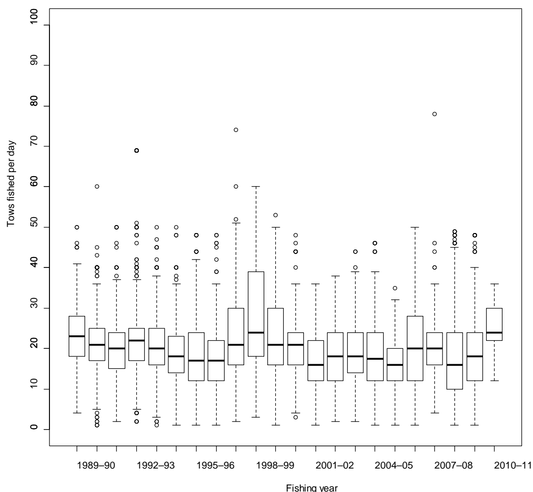
Figure 5: The distribution of the number of tows reported for each day's fishing, by fishing year.
