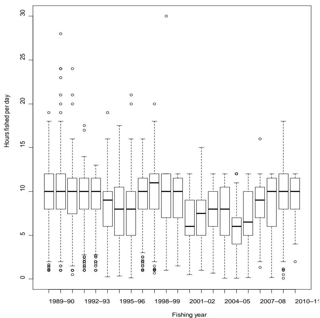
Figure 4: The distribution of reported estimates of the number of hours fished per day, by fishing year.
