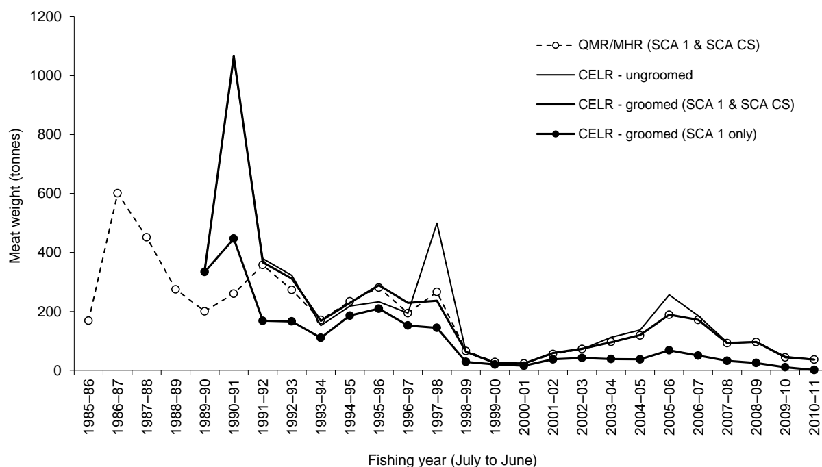
Figure 3: Comparison of annual catch totals derived from ungroomed and groomed Catch Effort Landing Return (CELRL) data relative to totals derived from Quota Management Returns (QMRs) and Monthly Harvest Returns (MHRs).
