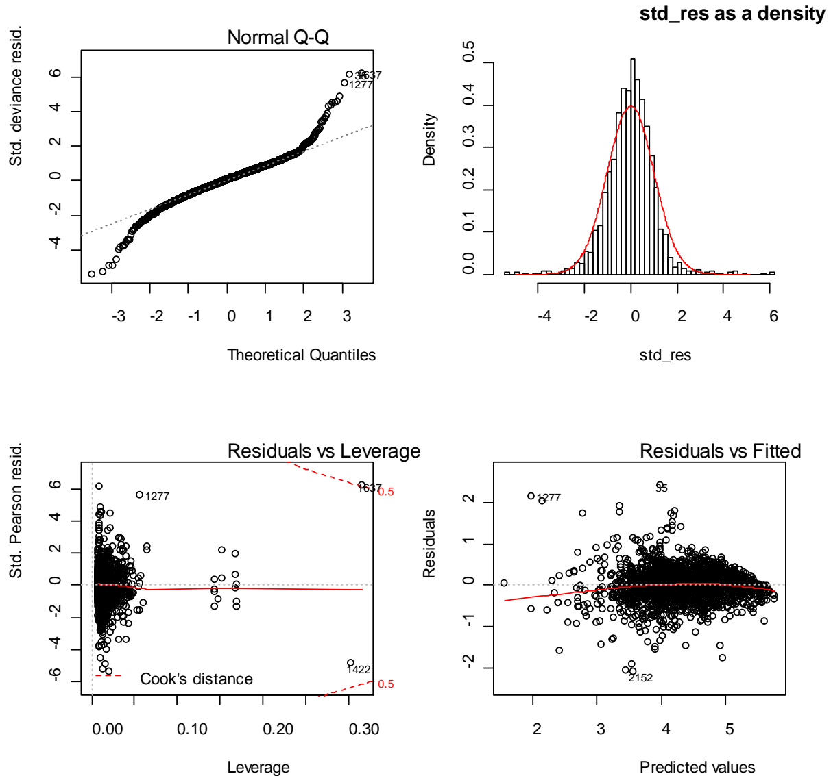
Figure C1: Diagnostic plots describing the fit of a standardised model of scallop catch rates for the Bream Bay scallop fishery. A quantile-quantile plot of standardised residuals [upper left panel]; a histogram of the standardised residuals compared to the distribution predicted from a lognormal distribution [upper right panel]; a plot of standardised residuals against the leverage that each data point has on the modelled relationship between daily catches and explanatory variables [lower left panel]; standardised residuals plotted against predicted daily catches [lower right panel].
