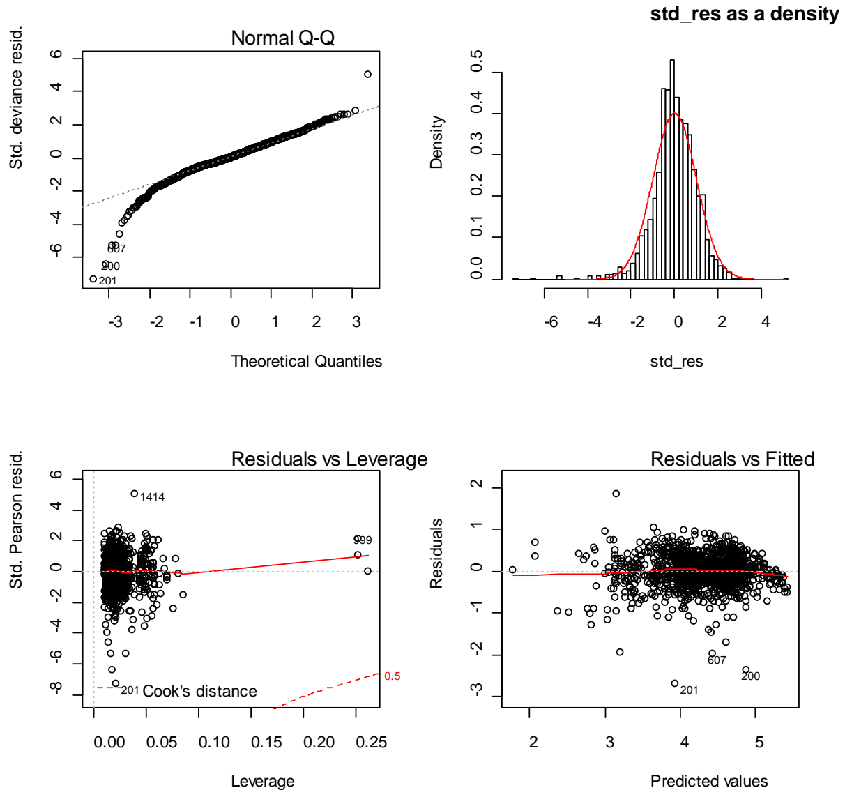
Figure D1: Diagnostic plots describing the fit of a standardised model of scallop catch rates for the Spirits Bay scallop fishery. A quantile-quantile plot of standardised residuals [upper left panel]; a histogram of the standardised residuals compared to the distribution predicted from a lognormal distribution [upper right panel]; a plot of standardised residuals against the leverage that each data point has on the modelled relationship between daily catches and explanatory variables [lower left panel]; standardised residuals plotted against predicted daily catches [lower right panel].
