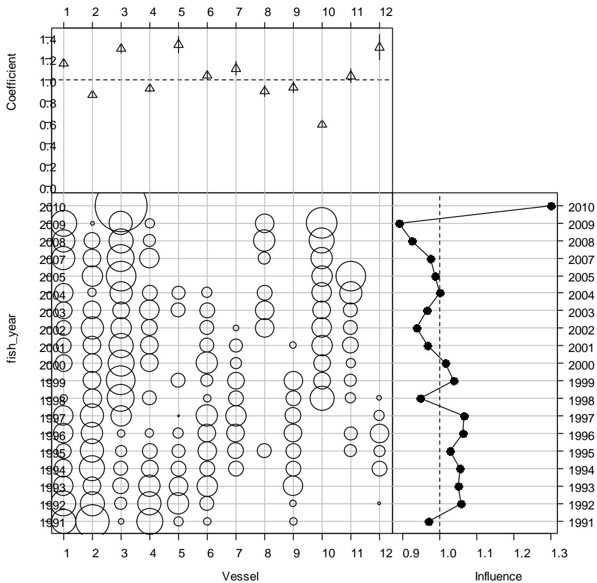
Figure B3: Effect of individual vessels on a lognormal model of daily catches in Rangaunu Bay. Effect by vessel [upper panel]; Distribution of observations by fishing year [lower left panel]; cumulative effect of the variable vessel by fishing year [lower right panel].
