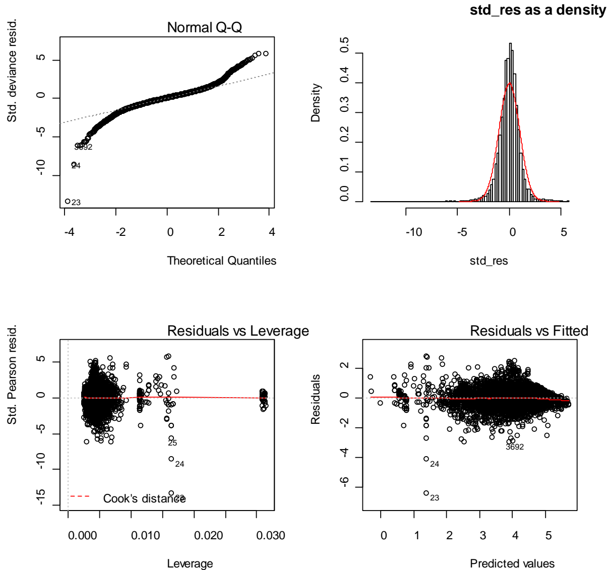
Figure E1: Diagnostic plots describing the fit of a standardised model of scallop catch rates for all three areas combined. A quantile-quantile plot of standardised residuals [upper left panel]; a histogram of the standardised residuals compared to the distribution predicted from a lognormal distribution [upper right panel]; a plot of standardised residuals against the leverage that each data point has on the modelled relationship between daily catches and explanatory variables [lower left panel]; standardised residuals plotted against predicted daily catches [lower right panel].
