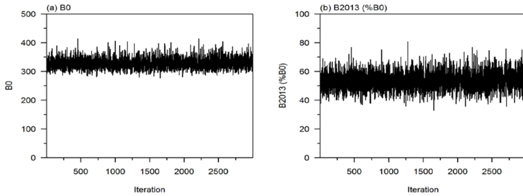
Figure 8: MCMC posterior trace plots for (a) B_0 and (b) current biomass ( \%B_{2013}/B_0 ) for run 1.2.
