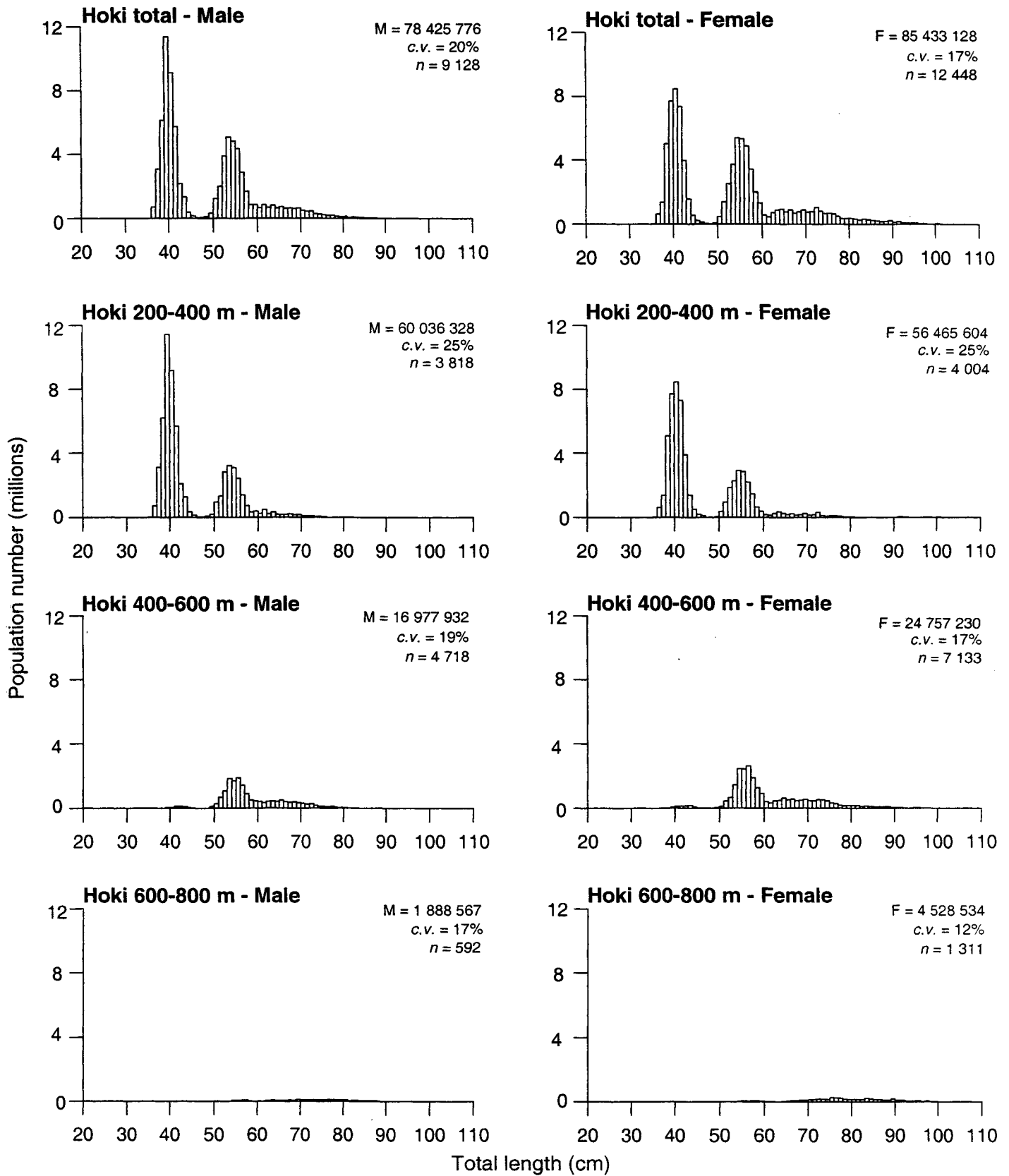
Figure 5a: Scaled length frequencies for hoki, by sex and depth zone (200-400, 400-600, 600-800m) (M, estimated male population; F, estimated female population; c.v., coefficient of variation of the estimated numbers of fish; n, numbers of fish measured)
