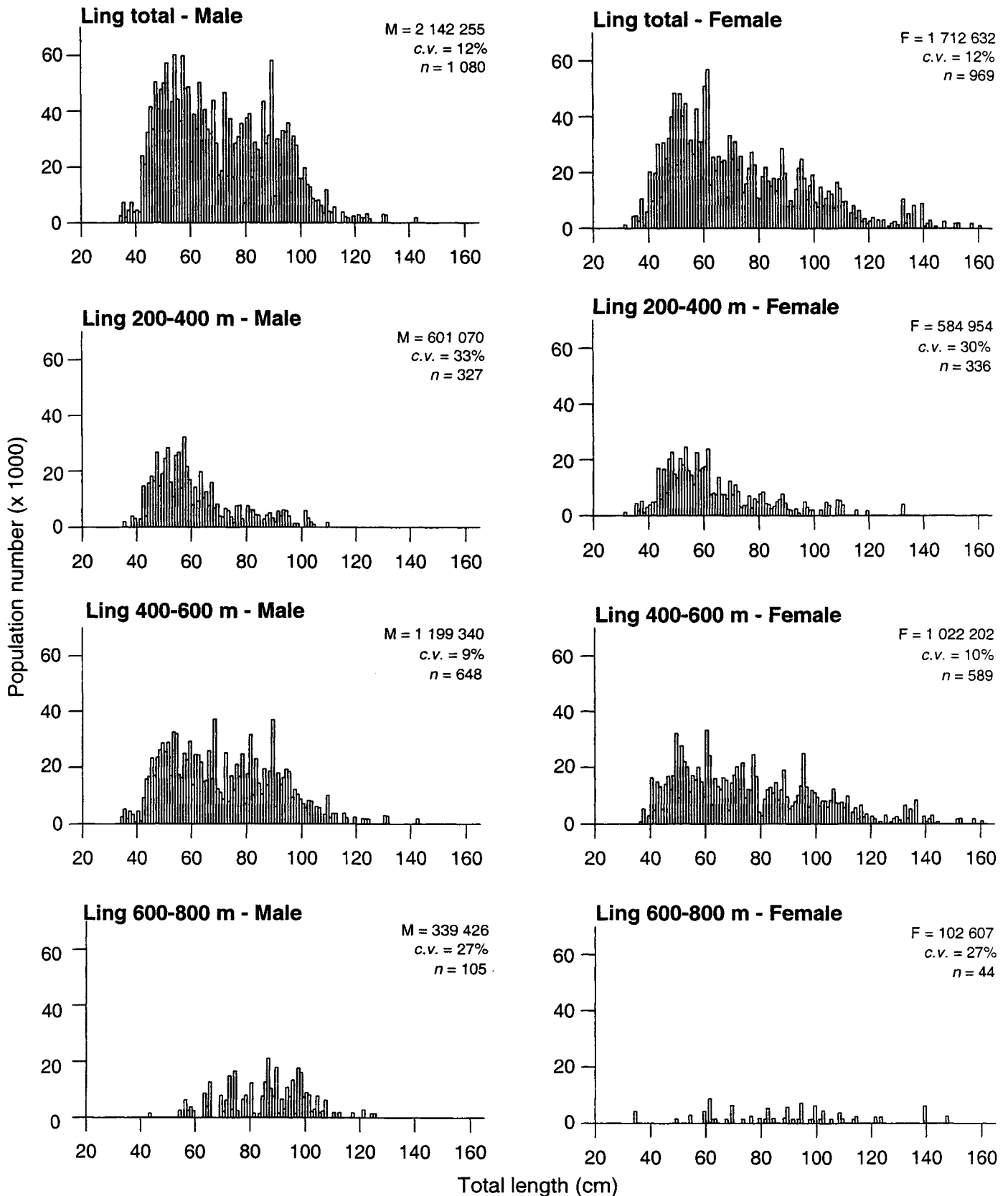
Figure 7: Scaled length frequencies for ling, by sex and depth zone (200-400, 400-600, 600-800m) (M, estimated male population; F, estimated female population; c.v., coefficient of variation of the estimated numbers of fish; n, numbers of fish measured)
