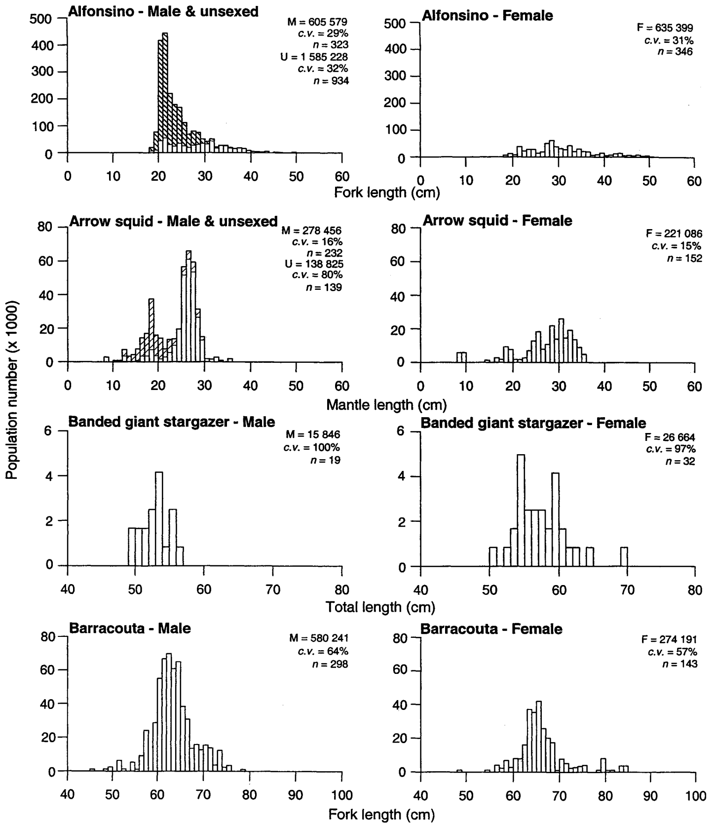
Figure 8: Scaled length frequencies for the major species, by sex (M, estimated male population; F, estimated female population; U, estimated unsexed population (hatched bars); c.v. coefficient of variation of the estimated numbers of fish; n, number of fish measured)
