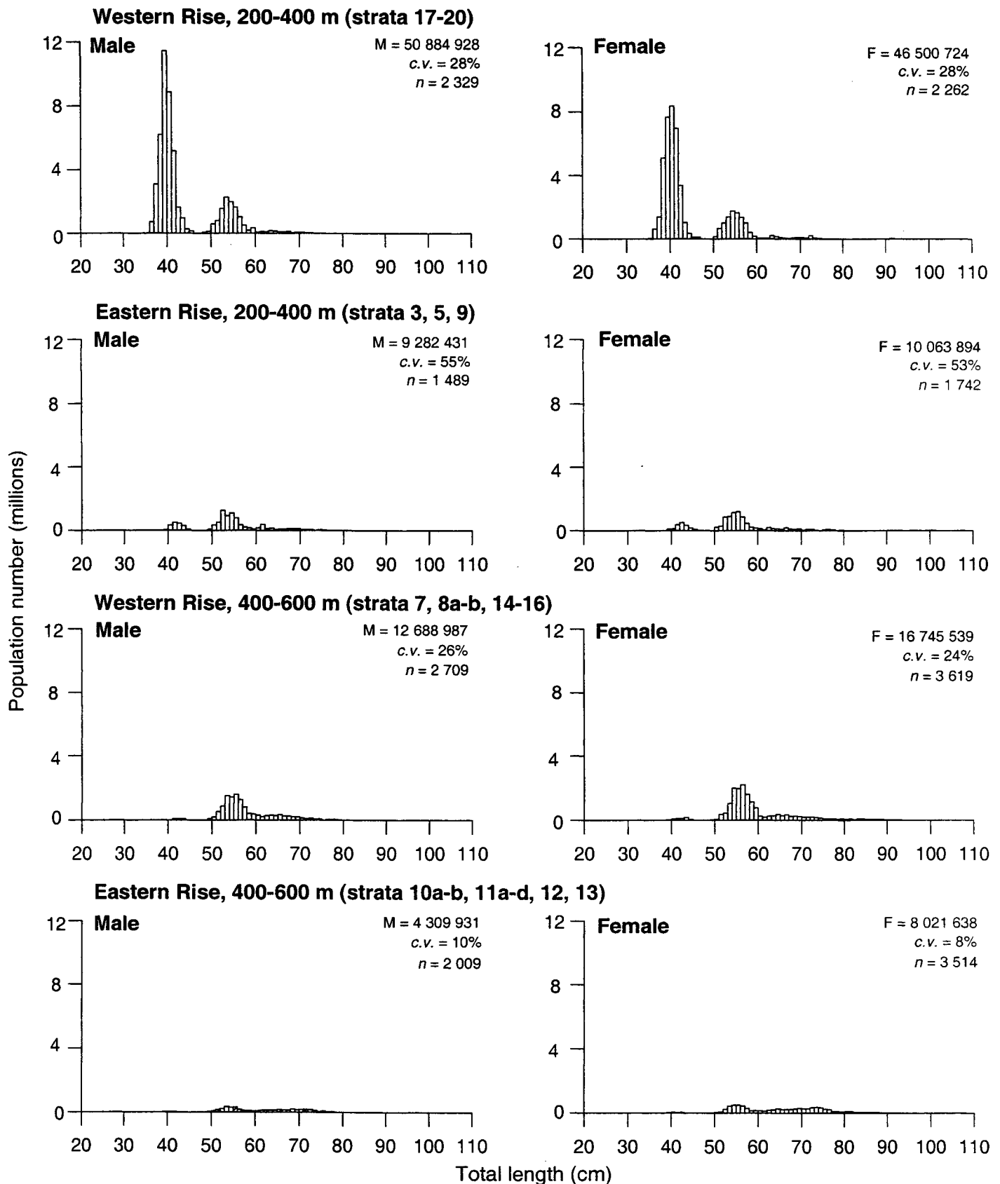
Figure 5b: Scaled length frequencies for hoki, by sex and depth zone (200-400, 400-600, 600-800m) (M, estimated male population; F, estimated female population; c.v., coefficient of variation of the estimated numbers of fish; n, numbers of fish measured)
