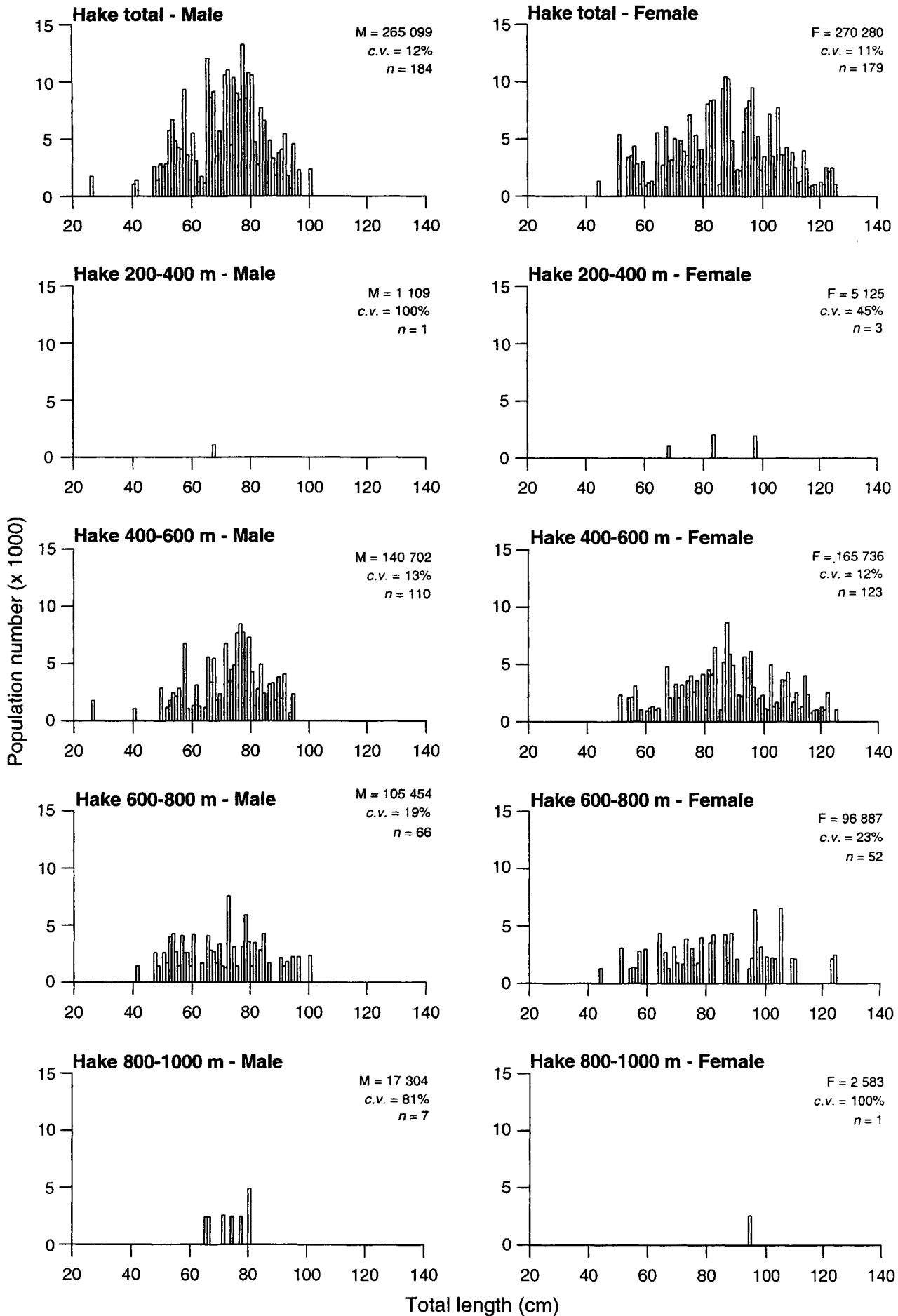
Figure 6: Scaled length frequencies for hake, by sex and depth zone (200-400, 400-600, 600-800, 800-1000m) (M, estimated male population; F, estimated female population; c.v., coefficient of variation of the estimated numbers of fish; n, number of fish measured)
