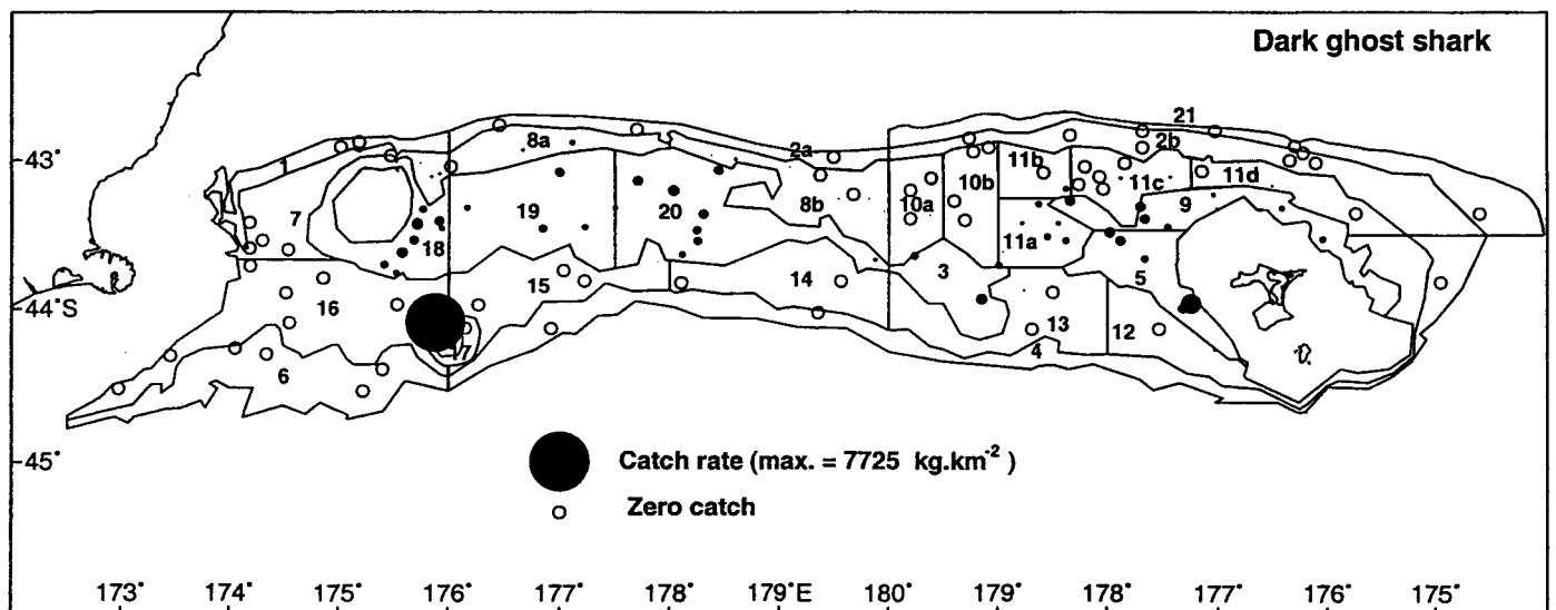
Figure 4: Catch rates (kg.km -2 ) of the most abundant species (after hoki). Circle area is proportional to catch rate. (max., maximum catch rate)
