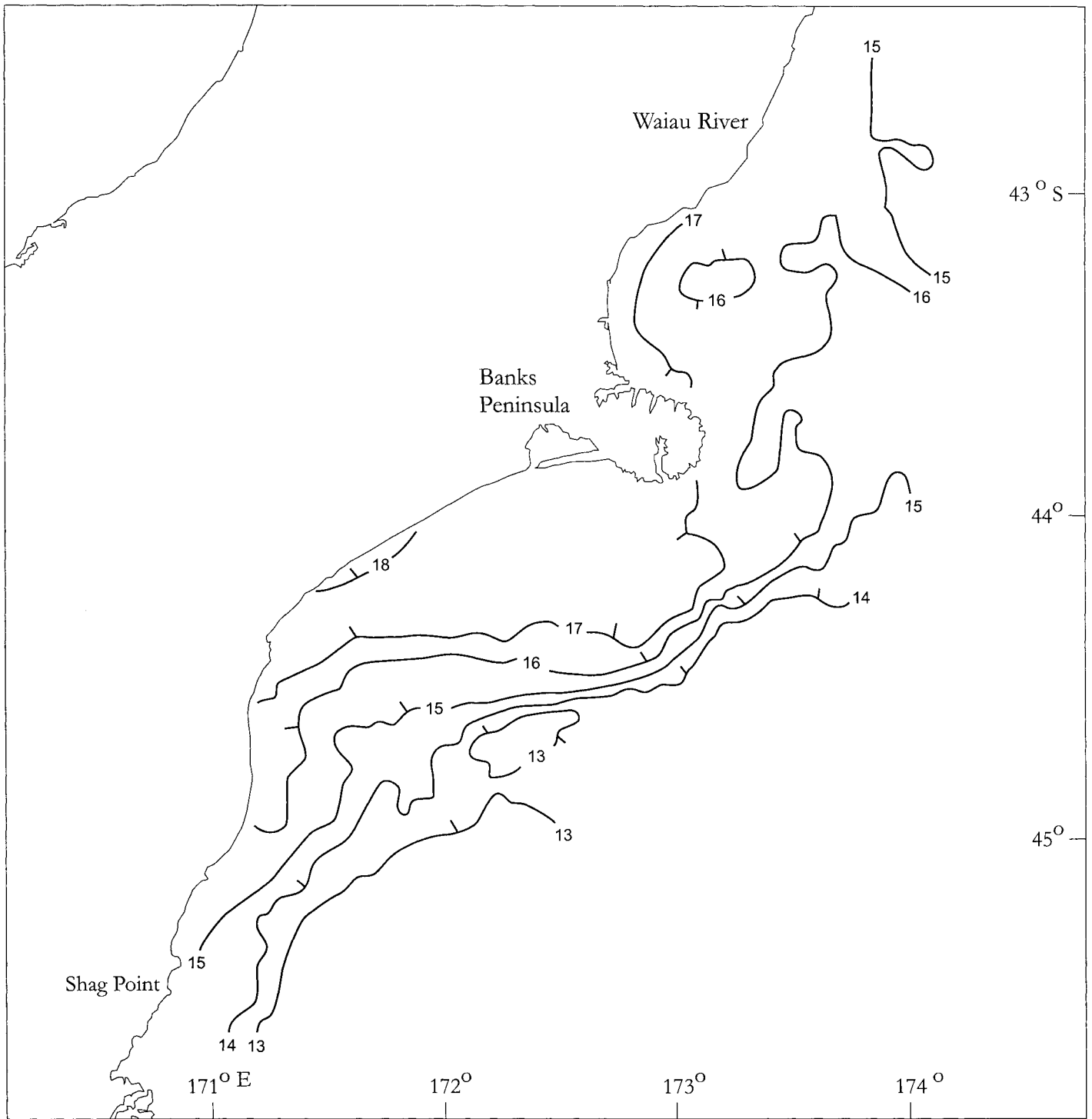
Figure 3: Mean sea surface isotherms for 9 – 11 January 1999 (from the NIWA SST Archive).
