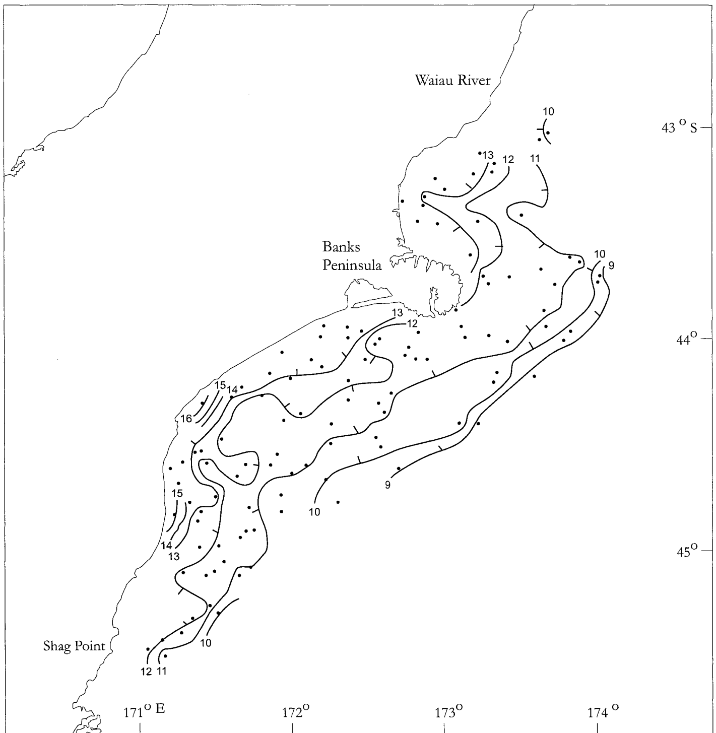
Figure 2: Positions of bottom temperature recordings and isotherms estimated from these data.
