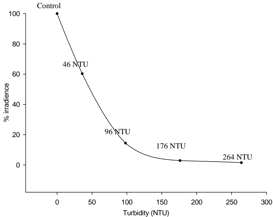
Figure 6: The irradiance of photosynthetically active light (PAR) at the surface of the sediment plotted against turbidity in different suspended sediment concentrations, relative to that in the control treatment.
