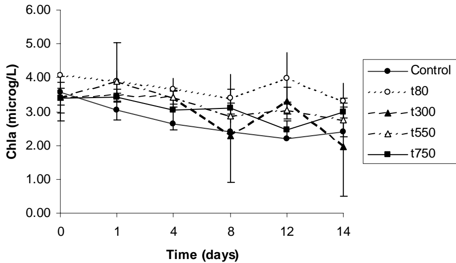
Figure 8: Chlorophyll a content of sediment (microg/L) in Echinocardium experimental aquaria (mean +/- 1 sd).
