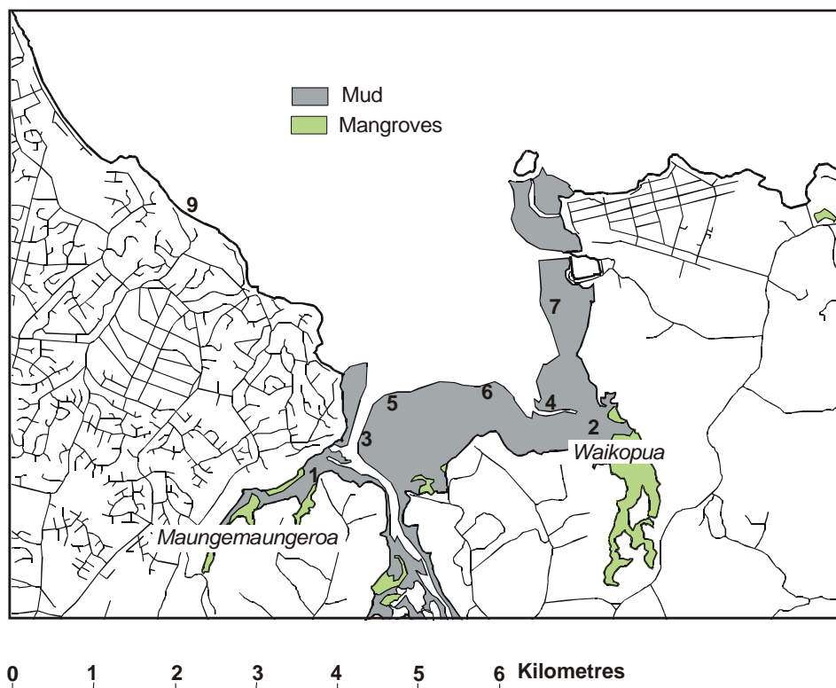
Figure 1: Map of the Whitford embayment showing the positions of optical backscatter sensors, May 2001 (Hewitt et al. 2001).
