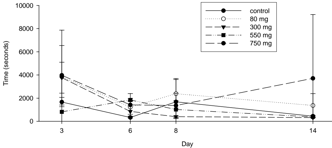
Figure 10: Time (seconds) taken for Macomona to bury (mean \pm 1 sd).
