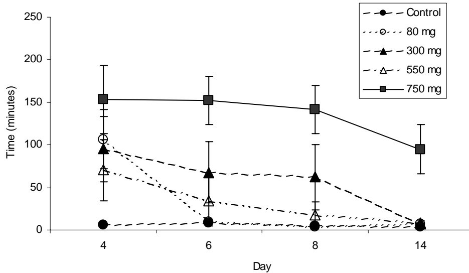
Figure 9: Time (minutes) taken for Echinocardium to re-bury (mean \pm 1 sd). Individuals who did not bury in 3 hours, were given a value of 180 minutes.
