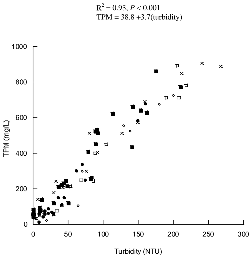
Figure 5: Relationship between turbidity (NTU) and suspended sediment concentrations (TPM). Data from the different experiments are shown as different symbols.
