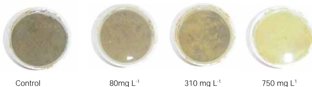
Figure 4: Plastic containers with sediment and Boccardia . Each container was 13 cm wide by 8 cm deep. Note the change in water clarity with increasing suspended sediment concentrations, from left to right.
