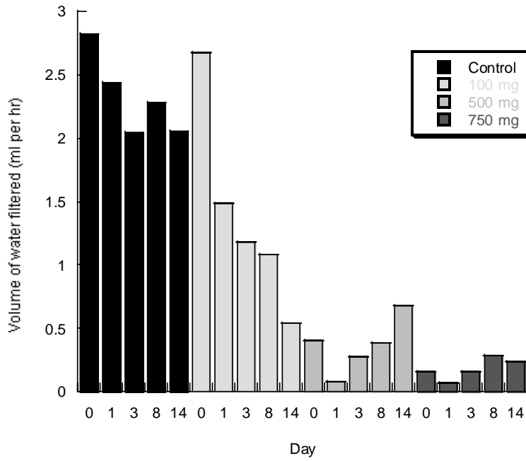
Figure 11: The volume of water filtered by Pecten over time (ml hr -1 ).
