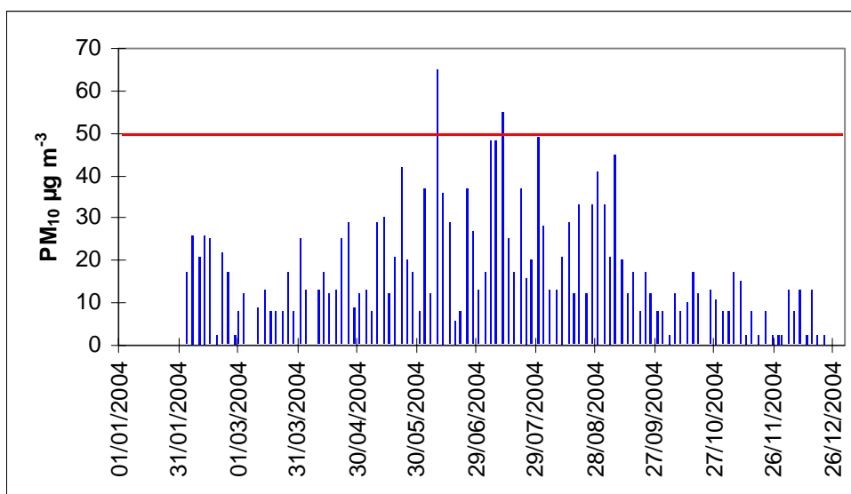
Figure 4-1: 24-hour average concentrations of PM 10 in Taupo during 2004
