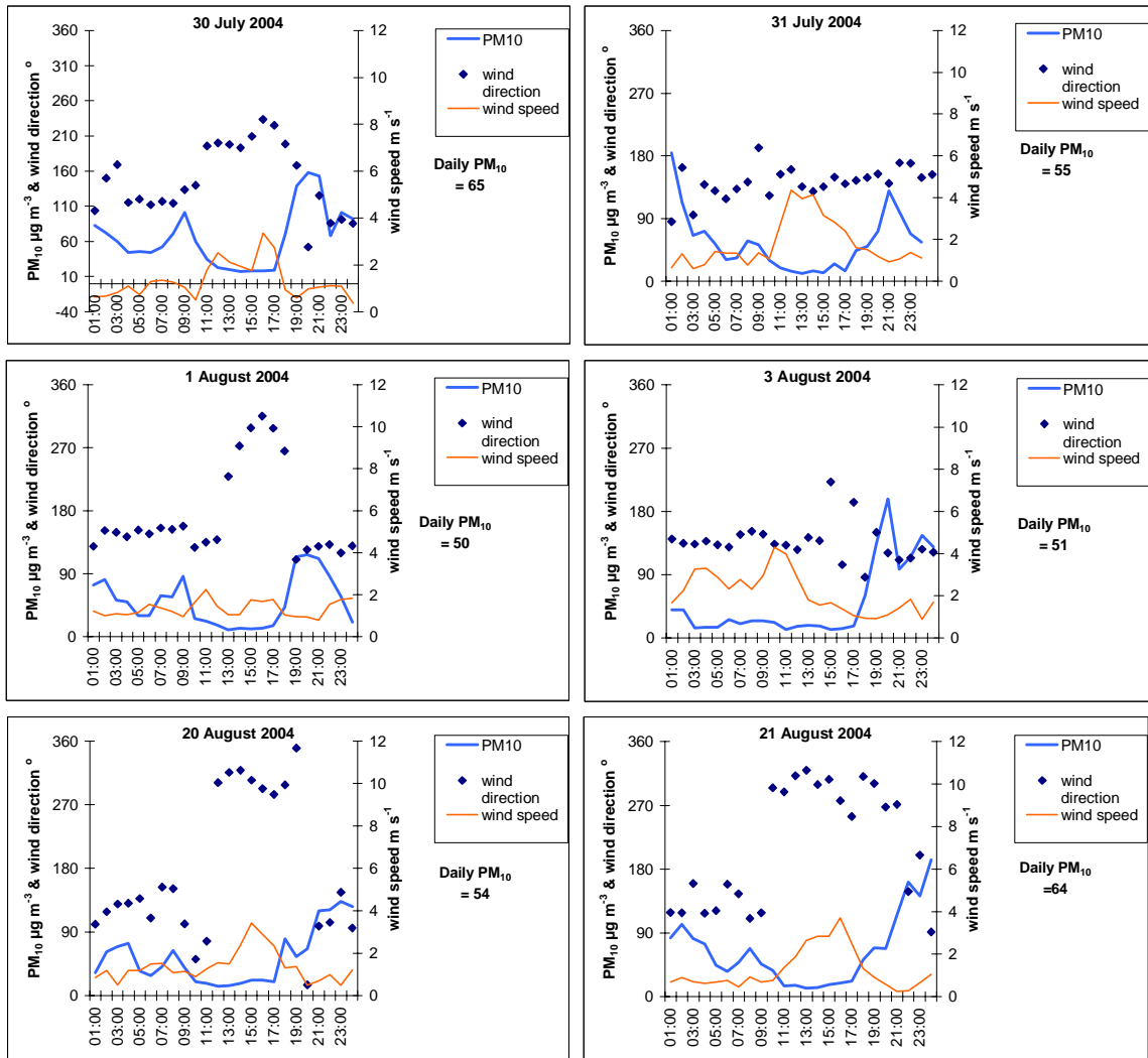
Figure 3-9: Daily variations in PM10, wind direction and wind speed on days the guideline was exceeded from 27 July to 21 August 2004
