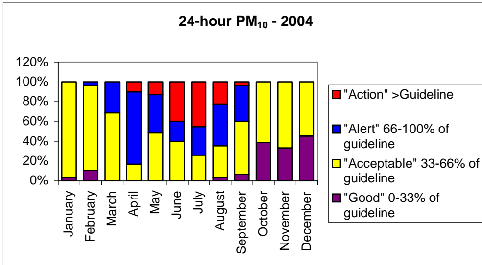
Figure 3-2: Comparison of PM 10 concentrations measured in Tokoroa to MfE air quality indicator categories
