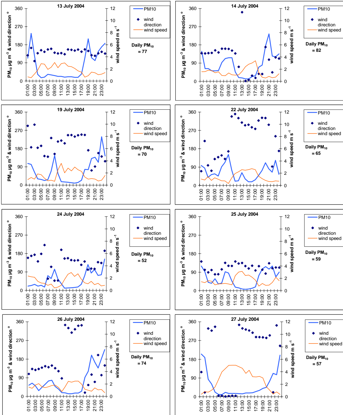
Figure 3-8: Daily variations in PM10, wind direction and wind speed on days the guideline was exceeded from 12 to 27 July 2004
