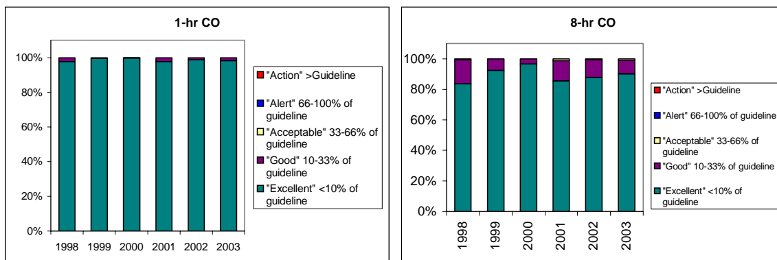
Figure 2-9: Comparison of CO concentrations measured in Hamilton from 1998 to 2004 to MfE air quality indicator categories
