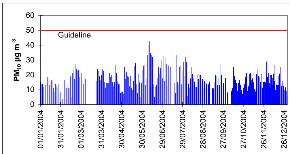
Figure 2-1: Daily PM10 concentrations measured in Hamilton during 2004
