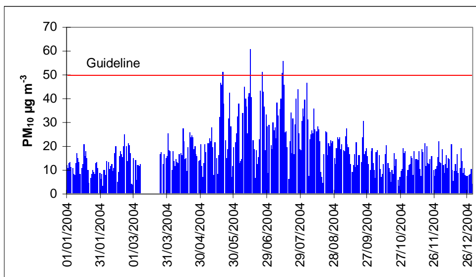
Figure 5-1: 24-hour average concentrations of PM10 in Te Kuiti during 2004
