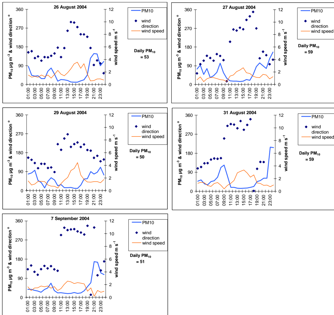
Figure 3-10: Daily variations in PM10, wind direction and wind speed on days the guideline was exceeded from 22 August to 7 September 2004
