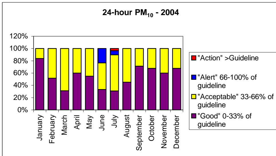
Figure 2-3: Comparison of PM10 concentrations measured in Hamilton during 2004 to MfE air quality indicator categories
