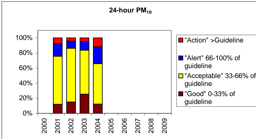
Figure 3-3: Comparison of PM10 concentrations measured in Tokoroa from 2001 to 2004 to MfE air quality indicator categories
