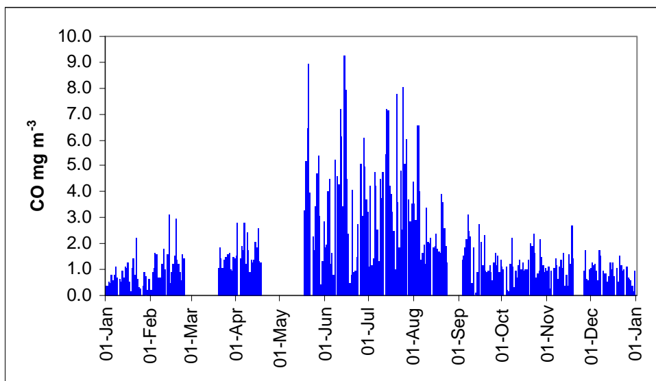
Figure 2-6: Concentrations of CO (hourly average) measured in Hamilton during 2004
