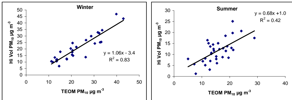
Figure 2-2: Comparison of PM10 concentrations measured using TEOM and high-volume sampler during 2004
