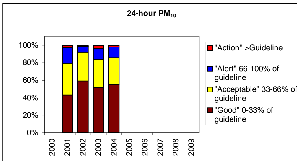
Figure 4-3: Comparison of PM10 concentrations measured in Taupo from 2001 to 2004 to MfE air quality indicator categories
