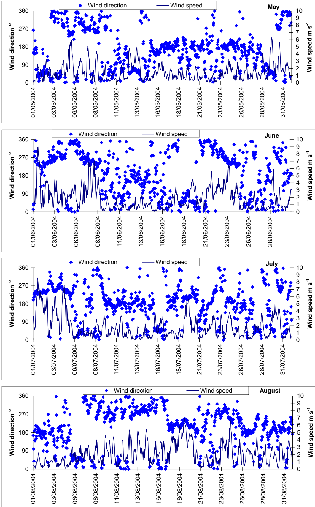
Figure 2-10: Hourly average wind direction and wind speed data for Hamilton from May to August 2004
