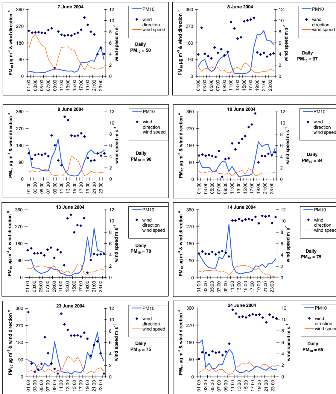
Figure 3-6: Daily variations in PM10, wind direction and wind speed on days the guideline was exceeded during 26 May to 24 June 2004
