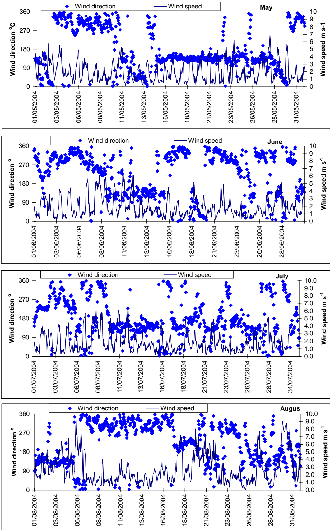
Figure 3-11: Hourly average wind direction and wind speed data for Tokoroa from May to August 2004
