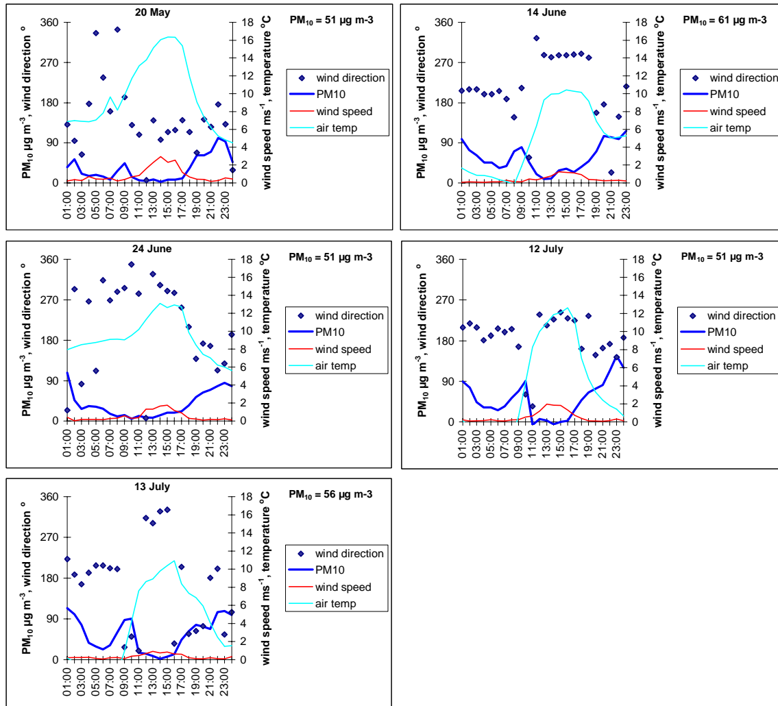
Figure 5-3: Daily variations in PM 10 , wind direction and wind speed on days the guideline was exceeded at Te Kuiti during 2004
