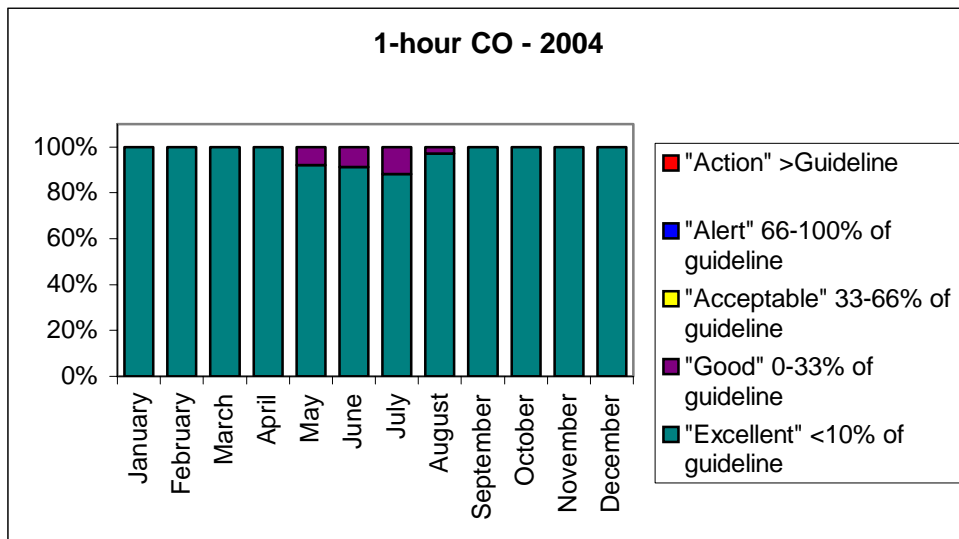
Figure 2-8: Comparison of 1-hour average CO concentrations measured in Hamilton during 2004 to MfE air quality indicator categories
