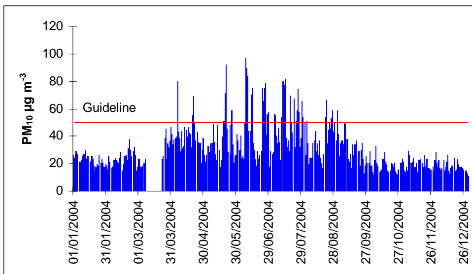
Figure 3-1: 24-hour average concentrations of PM10 in Tokoroa during 2004
