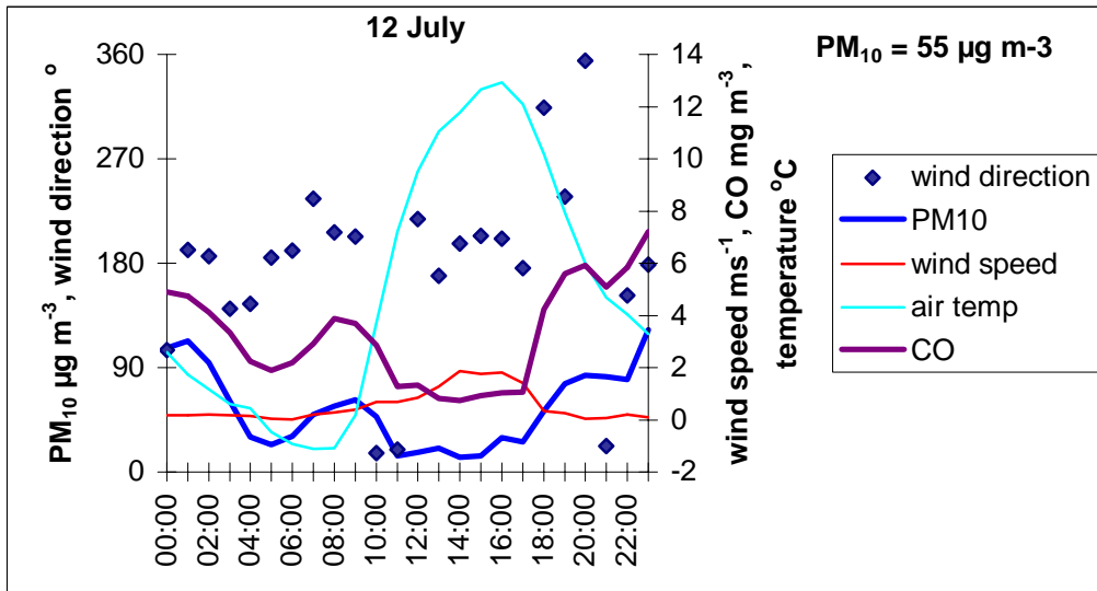
Figure 2-5: Daily variations in PM10, wind direction and wind speed on 12 July 2004
