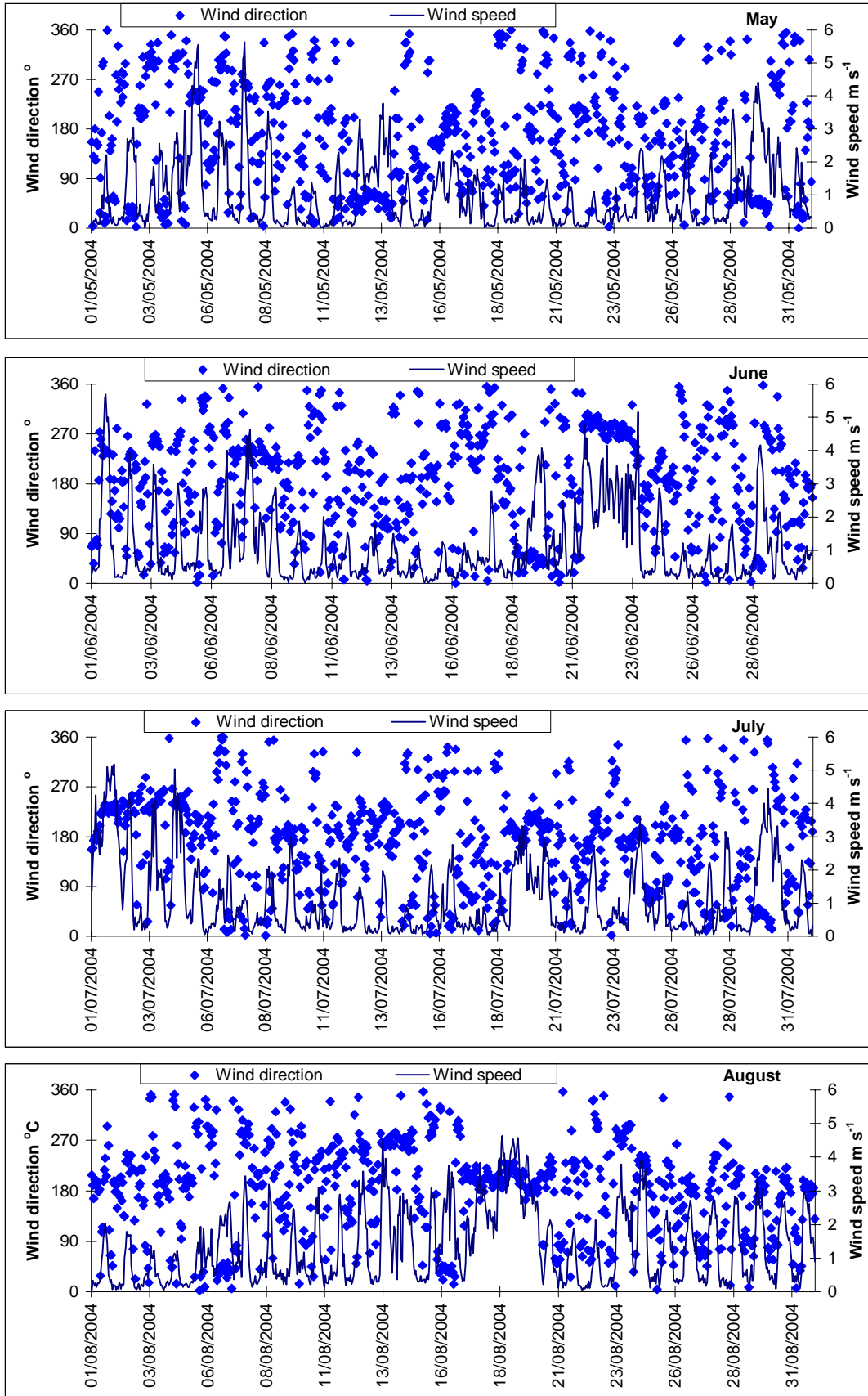
Figure 5-5: Hourly average wind direction and wind speed data for Te Kuiti from May to August 2004
