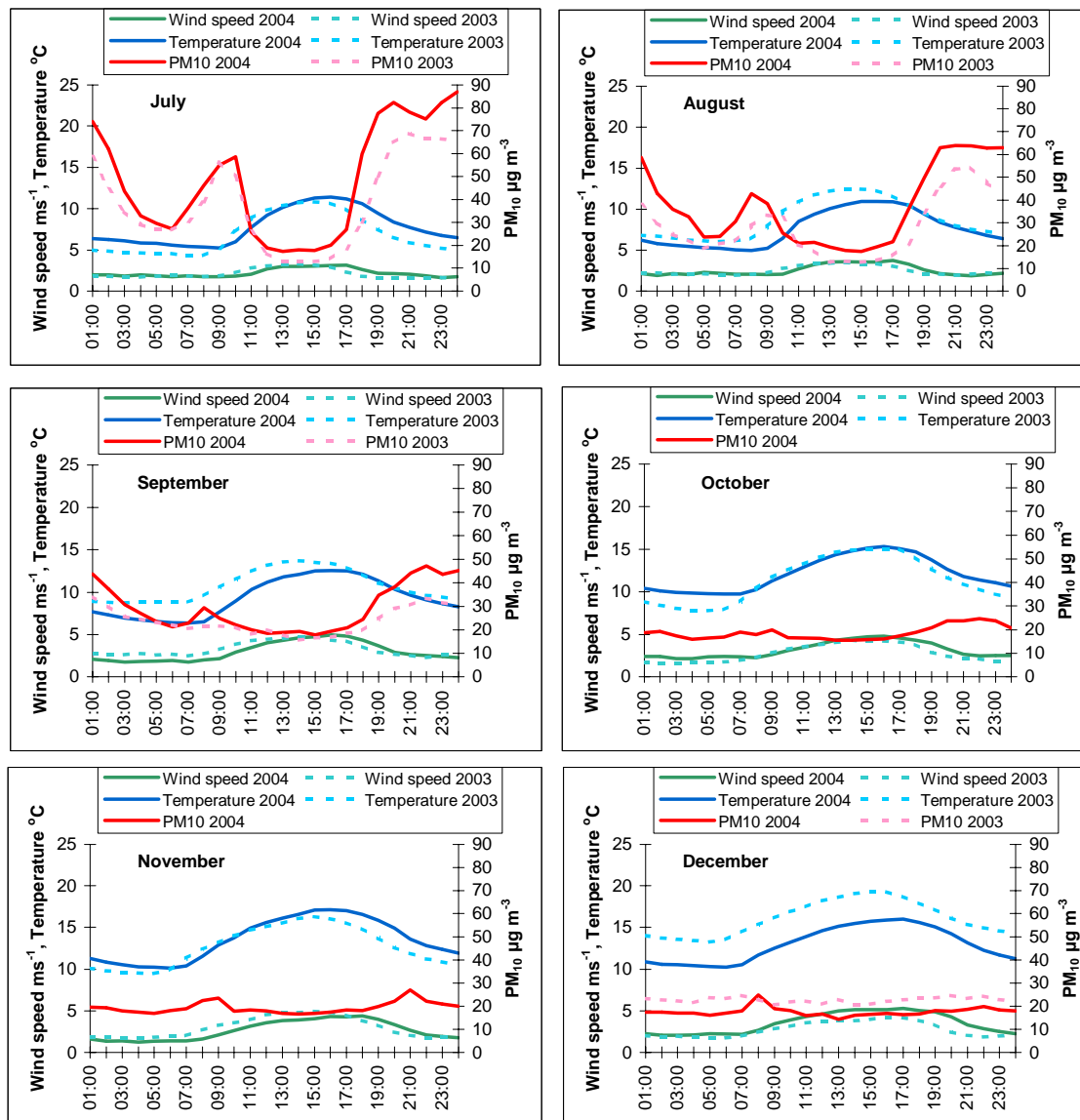
Figure 3-13: Hourly average PM 10 , wind speed and temperature values for 2003 and 2004 for each month from July to December
