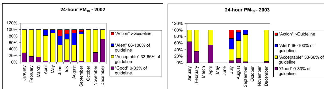
Figure 3-4: Seasonal variations in PM10 concentrations in Tokoroa during 2002 and 2003
