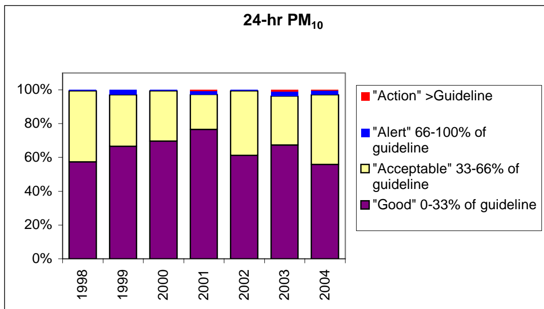
Figure 2-4: Comparison of PM10 concentrations measured at Hamilton from 1998 to 2004 to MfE air quality indicator categories
