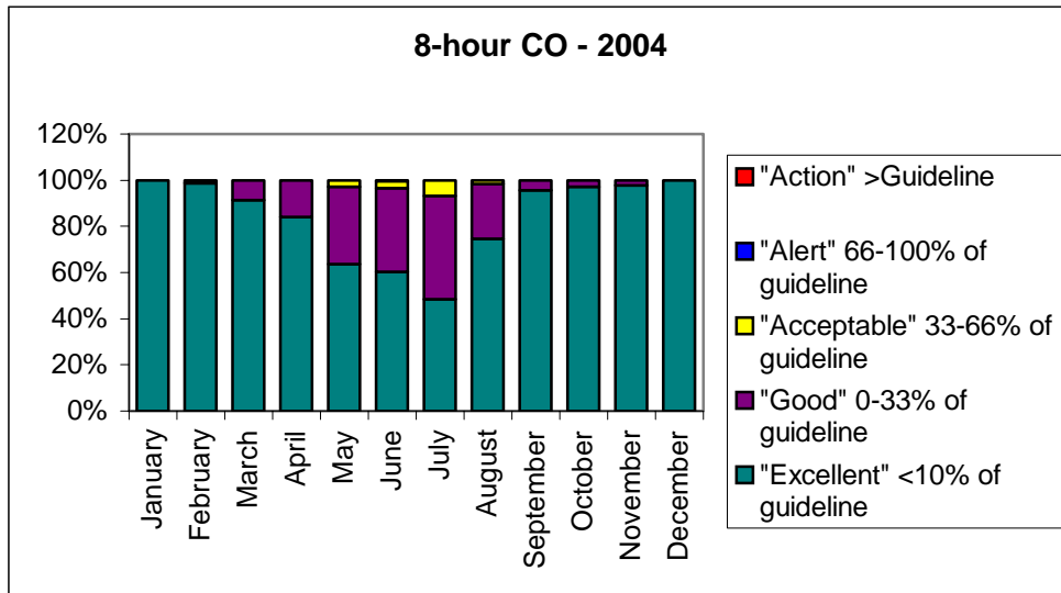
Figure 2-7: Comparison of 8-hour average CO concentrations measured in Hamilton during 2004 to MfE air quality indicator categories
