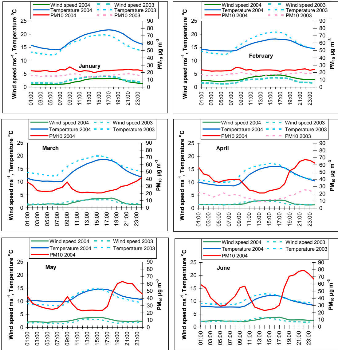
Figure 3-12: Hourly average PM10, wind speed and temperature values for 2003 and 2004 for each month from January to June
