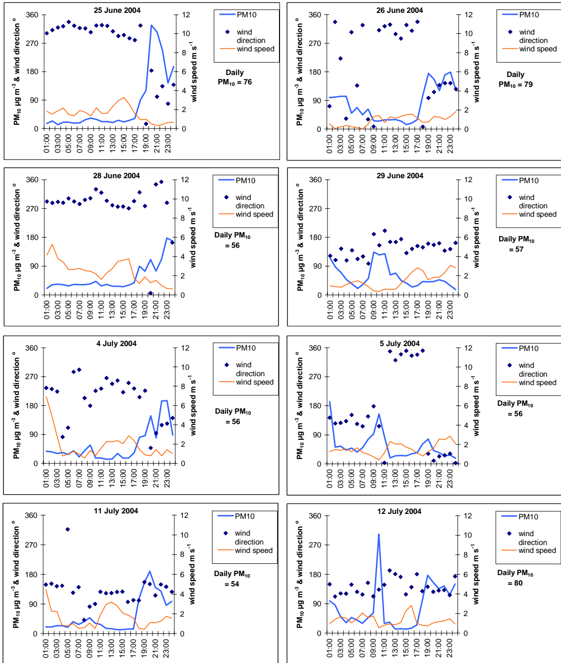
Figure 3-7: Daily variations in PM10, wind direction and wind speed on days the guideline was exceeded from 24 June to 12 July 2004
