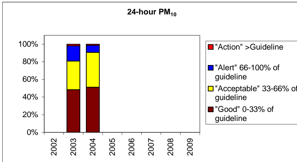
Figure 5-4: Comparison of PM 10 concentrations in Te Kuiti to MfE air quality indicator categories for 2003 and 2004
