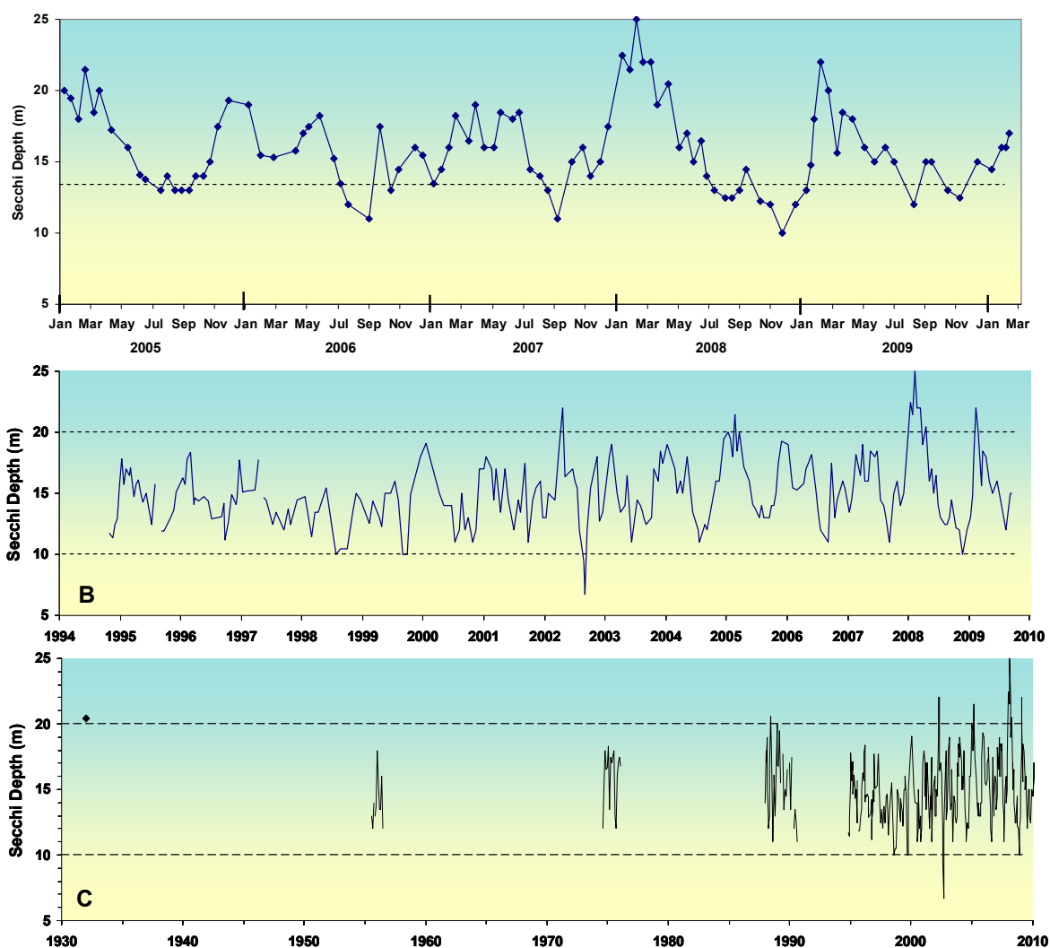
Figure 5: A) Time-series changes in water clarity as indicated by Secchi depth water clarity from summer 2005 through to winter 2009. Dotted line at 13.5 m is the mean winter water clarity for this period. Date ticks are 1 st of each month. B) Long-term changes in water clarity show the variability across seasons and years for the present monitoring programme since 1994. Date ticks are 1 st January each year. C) Combined Secchi depth record since 1932. The 1932 data point was from John S. Armstrong's notes after converting his value from feet to meters.
