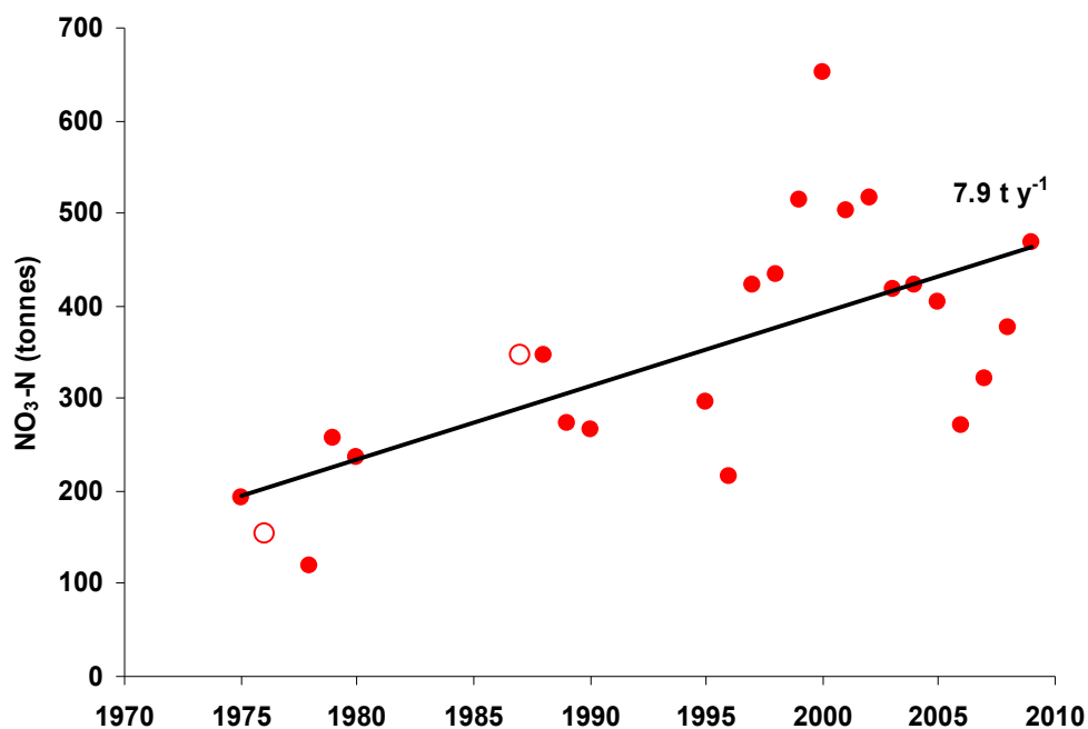
Figure 11: Long-term time series of total mass of NO 3 -N in the hypolimnion of Lake Taupo in autumn before winter mixing. The regression line indicates a statistically significant trend of increase in the total mass of 7.9 t y -1 ( P < 0.001 , r^2 = 0.41 , n = 22 ). Open circle data excluded from regression as time periods and depth data were not the same as used for the other data. Date ticks are 1 January in each year.
