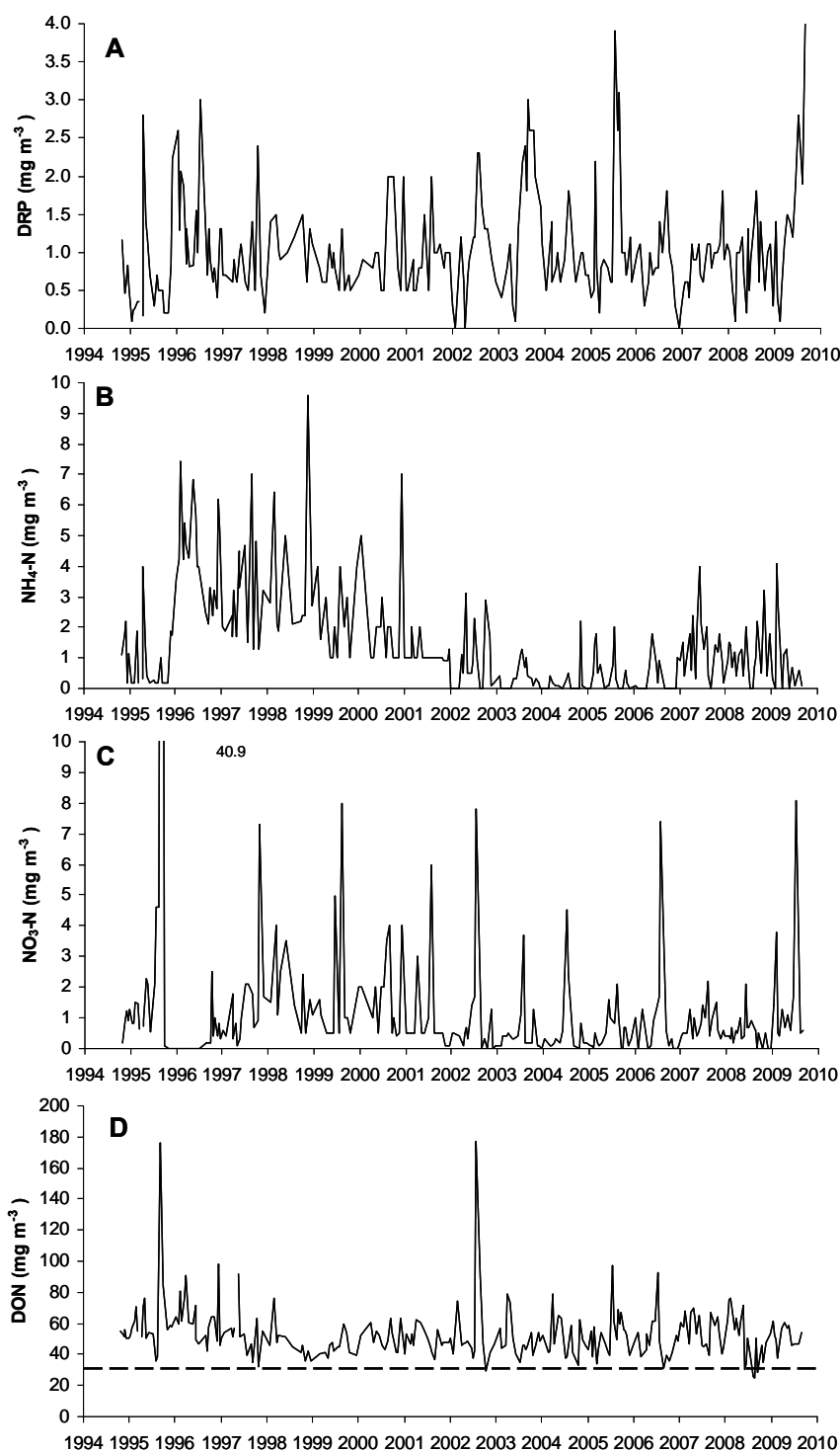
Figure 9: Time series data from the top 10 m of water column in Lake Taupo for (A) dissolved reactive phosphorus (DRP), (B) ammoniacal nitrogen ( \text{NH}_4\text{-N} ), (C) nitrate + nitrite nitrogen ( \text{NO}_3\text{-N} ), and (D) dissolved organic nitrogen (DON). Broken line indicates the “minimum” DON concentration, which may be the concentration of refractory organic material in the lake. Date ticks are 1 January in each year.
