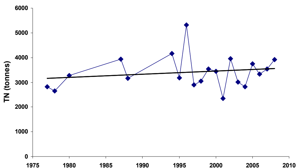
Figure 13: Long-term time series estimates of the mass of total nitrogen (TN) in Lake Taupo in spring after winter mixing. Although there is an average increase of about 12.9 \text{ t y}^{-1} over the data record, this apparent trend in the data is not statistically significant. The mean of the mass is around 3400 t. Date ticks are 1 January in each year.
