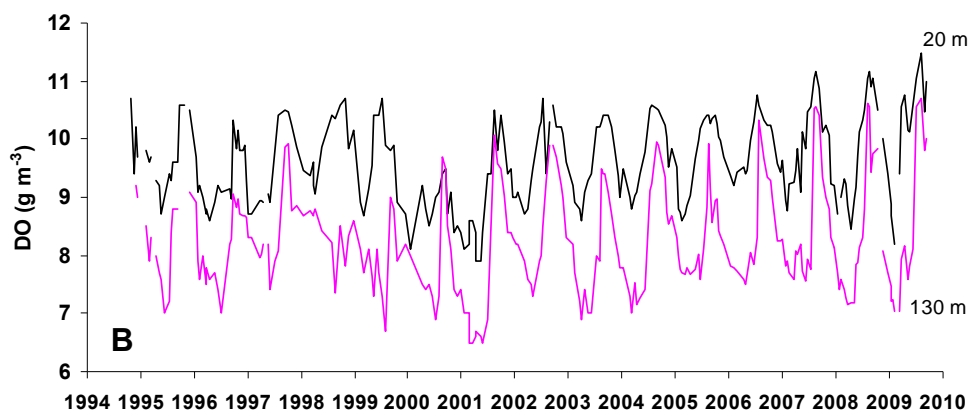
Figure 2B: Time-series dissolved oxygen data from 20 m (black line) and 130 m (pink line) depths. Mixing and complete reoxygenation occurred where the two lines in the temperature data (Fig. 2A) meet each winter. This corresponds with the period that the two lines on the oxygen data should meet. However, where temperature data indicate incomplete mixing and the 2 lines of the oxygen data do not meet, there is incomplete reoxygenation of the hypolimnion. Date ticks are 1 January in each year.
