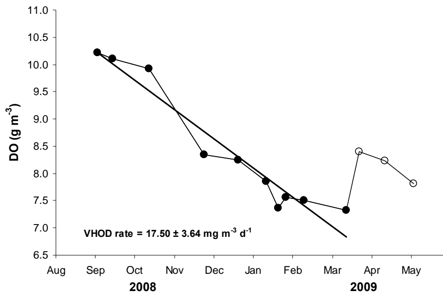
Figure 3: Volume-weighted mean dissolved oxygen (DO) concentrations below 70 m for 2008/09. The linear regression through the solid data points is the VHOD rate. ( P < 0.0001 , r^2 = 0.94 , n = 10 ).
