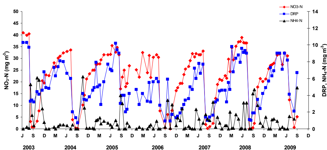
Figure 10: Time series data for DRP (blue square), \text{NO}_3\text{-N} (red diamond) and \text{NH}_4\text{-N} (black triangle) in the bottom waters (150 m depth) of Lake Taupo since winter mixing 2003.
