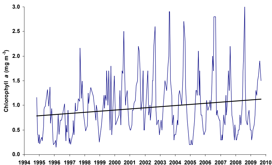
Figure 6: Time-series chlorophyll a concentrations in the upper 10 m of Lake Taupo at the mid-lake site, Site A. The solid regression line represents a statistically significant increase in the mean chlorophyll a concentrations of 0.025 \pm 0.017 \text{ mg m}^{-3} \text{ y}^{-1} ( P = 0.005 , r^2 = 0.03 , n = 237 ). Date ticks are 1 January in each year. Chlorophyll a detection limit = 0.1 \text{ mg m}^{-3} .
