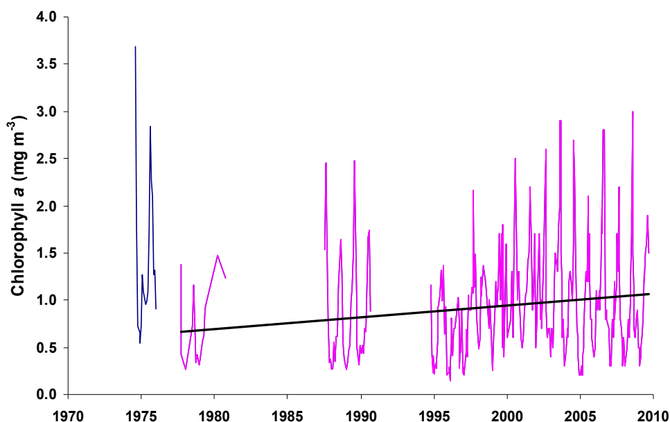
Figure 8: Time-series upper 10 m chlorophyll a concentrations in Lake Taupo from 1977 to present (pink). The 1974/75 data (blue) were collected by 30-m integrated tube sampler and are not directly comparable with the later data (See text). The linear regression line shows a statistically significant trend in the data from 1977 to present of 0.012 \pm 0.008 \text{ mg m}^{-3} \text{ y}^{-1} ( P < 0.005 , r^2 = 0.0265 , n = 304 ).
