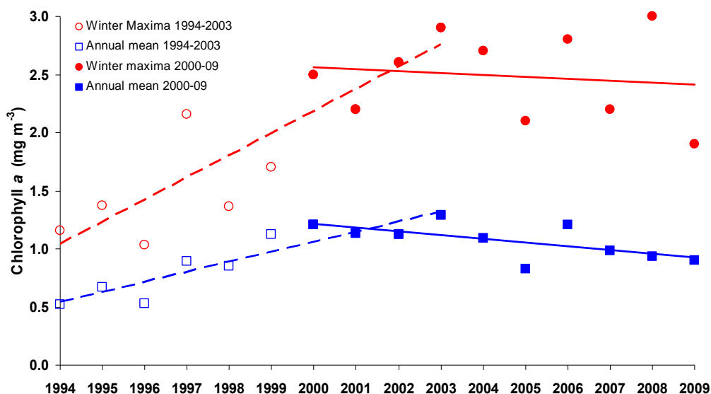
Figure 7: Annual average and winter maximum chlorophyll a concentrations from the 10-m tube samples since 1994. Regression lines indicate significant ( P < 0.001 ) trends of increase between 1994 and 2003 (broken lines) but trends of decrease from 2000 to 2009 (solid lines). These regressions use a data overlap between 2000 and 2003. Note the regression for the winter maxima decrease from 2000 to 2009 is not statistically significant ( P = 0.7 ). Regression slopes are as given in the text. Date ticks are 1 January in each year.
