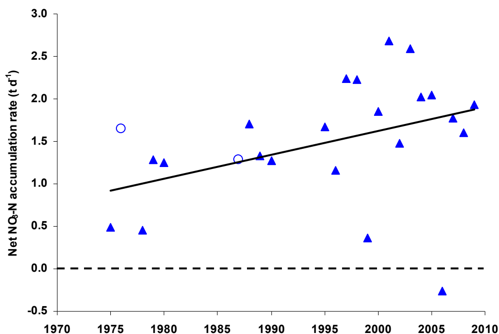
Figure 12: Net NO 3 -N accumulation rates (t d -1 ) in the hypolimnion below 70 m. The regression line shows an increase in the net accumulation rate of 0.028 \pm 0.03 t d -1 ( P = 0.07 , r^2 = 0.154 , n = 22 ). Open circle data were not included in the regression analysis (see text). Note that the Y-axis extends to -0.5 t d -1 for the 2006 data point. Date ticks are 1 January in each year.
