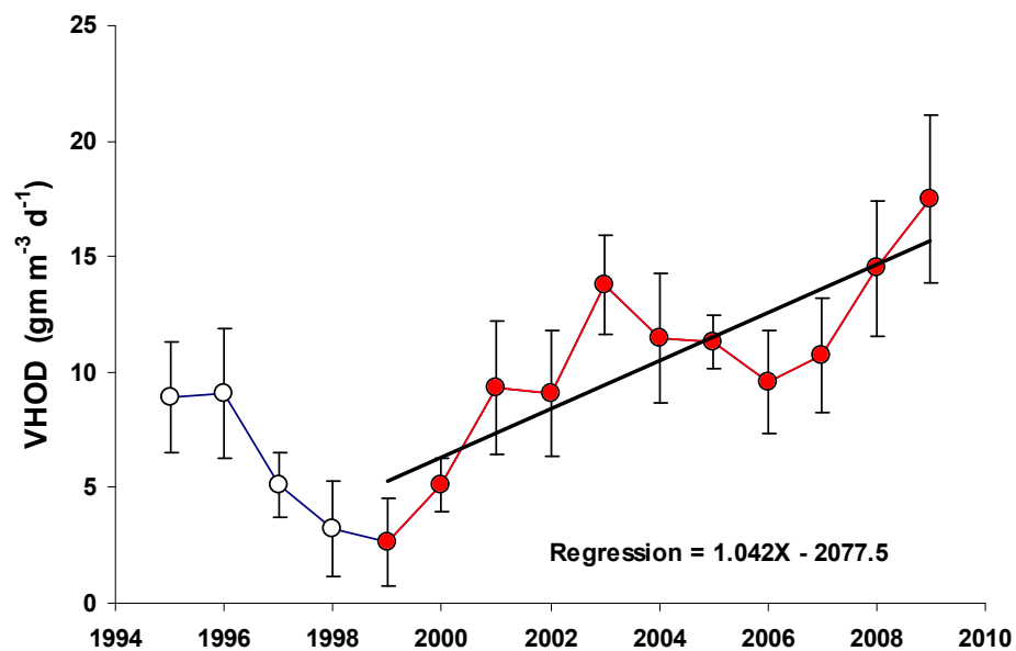
Figure 4: Time-series of VHOD rates since 1994-95. The low VHOD in 1997-2000 (following the 1995/96 eruptions of Mount Ruapehu) corresponds to a shift in algal dominance from diatoms to colonial greens ( Botryococcus braunii ). The regression through the solid (red) dots ( P < 0.002 , r^2 = 0.69 , n = 11 ), only looks at the change in VHOD since 1998/99, the lowest VHOD rate in the long term monitoring programme, and the beginning of the return of diatoms as the dominant algal species.
