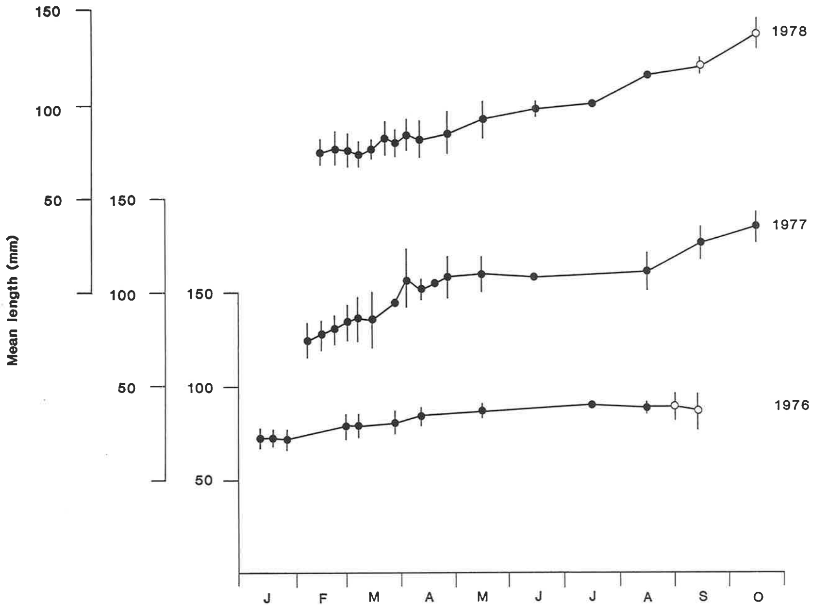
FIGURE 2. Mean length, with \pm 1 standard deviation, of chinook salmon fingerlings leaving the upper lake in various months, 1976-78. Open circles = fish taken out by netting. Standard deviation not shown where n < 5 .
